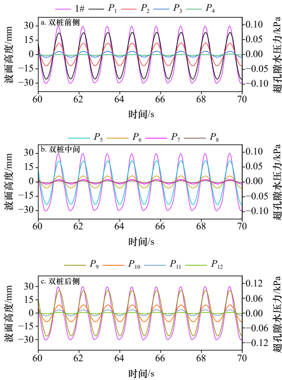
图9 动态对齐后波高与超孔压 Fig. 9 Wave height and excess pore pressure after dynamic alignment
